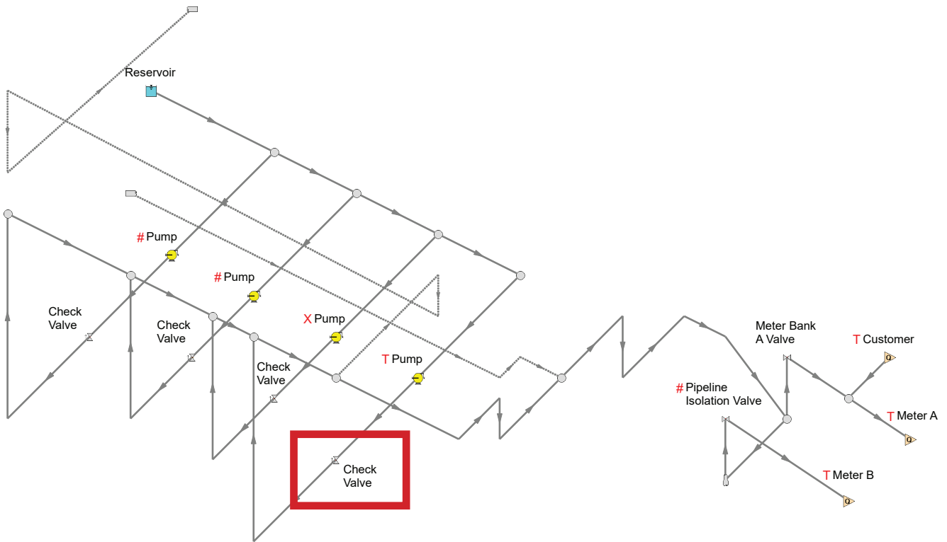
Figure 2 - AFT Impulse simulated the trip of a trial check valve slam to lower peak pressure
