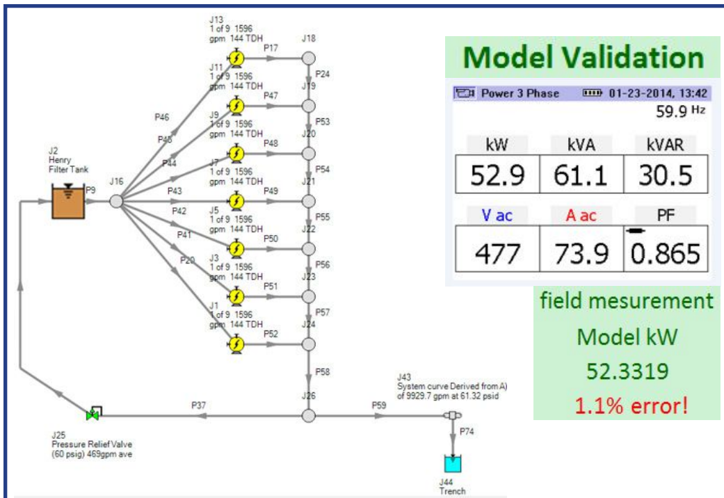
Figure 2 - System simulation: Dundee Engine North Head Line Coolant System; AFT Fathom model; Model validated to 1.1% of field measurements.
